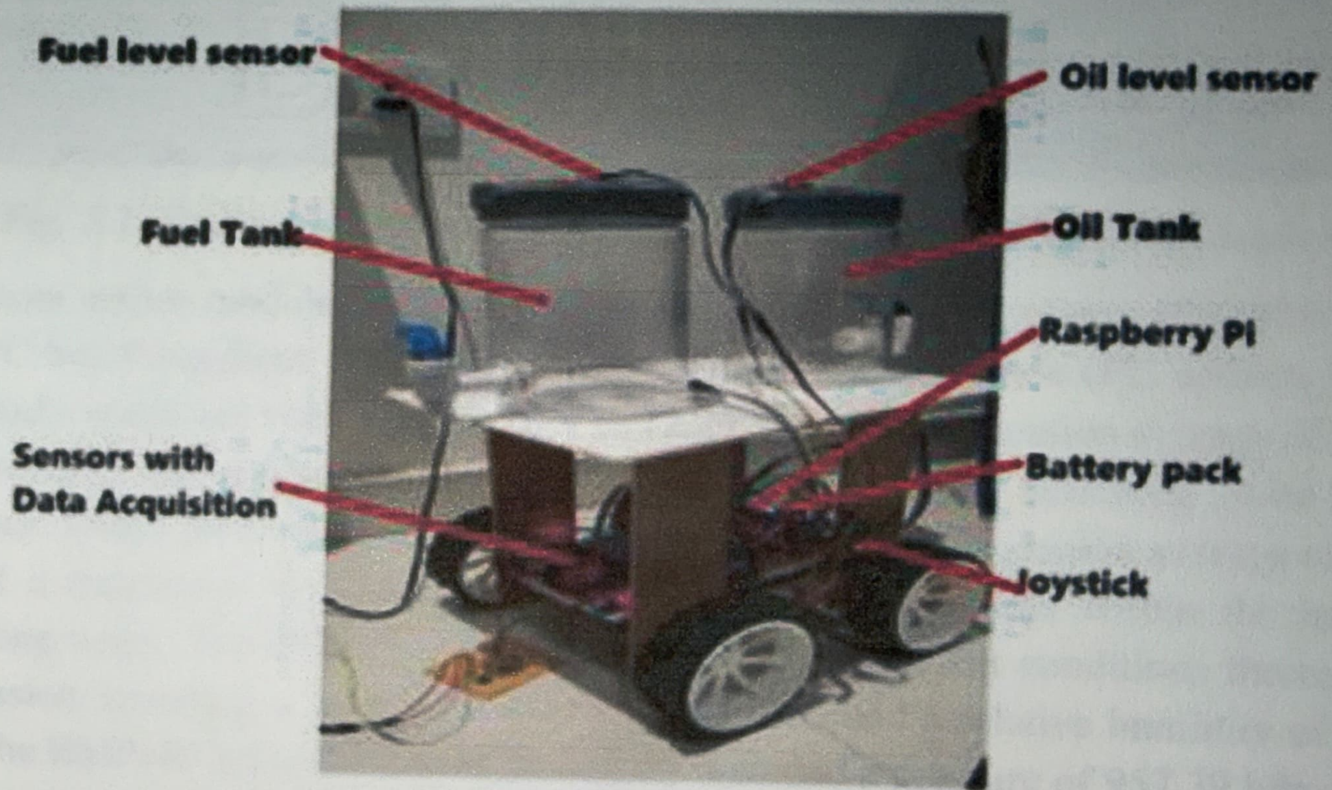
Fig. 5.1: Final Hardware Prototype of the Digital Twin Vehicle Health Monitoring System
